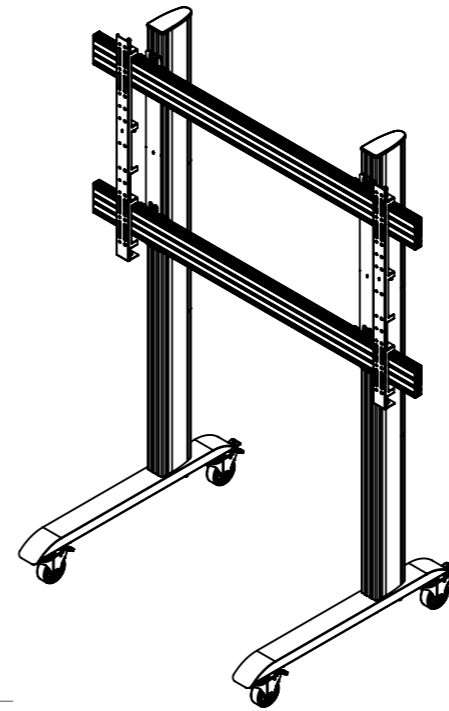
ISOMETRIC VIEW SCALE: 1 : 25
